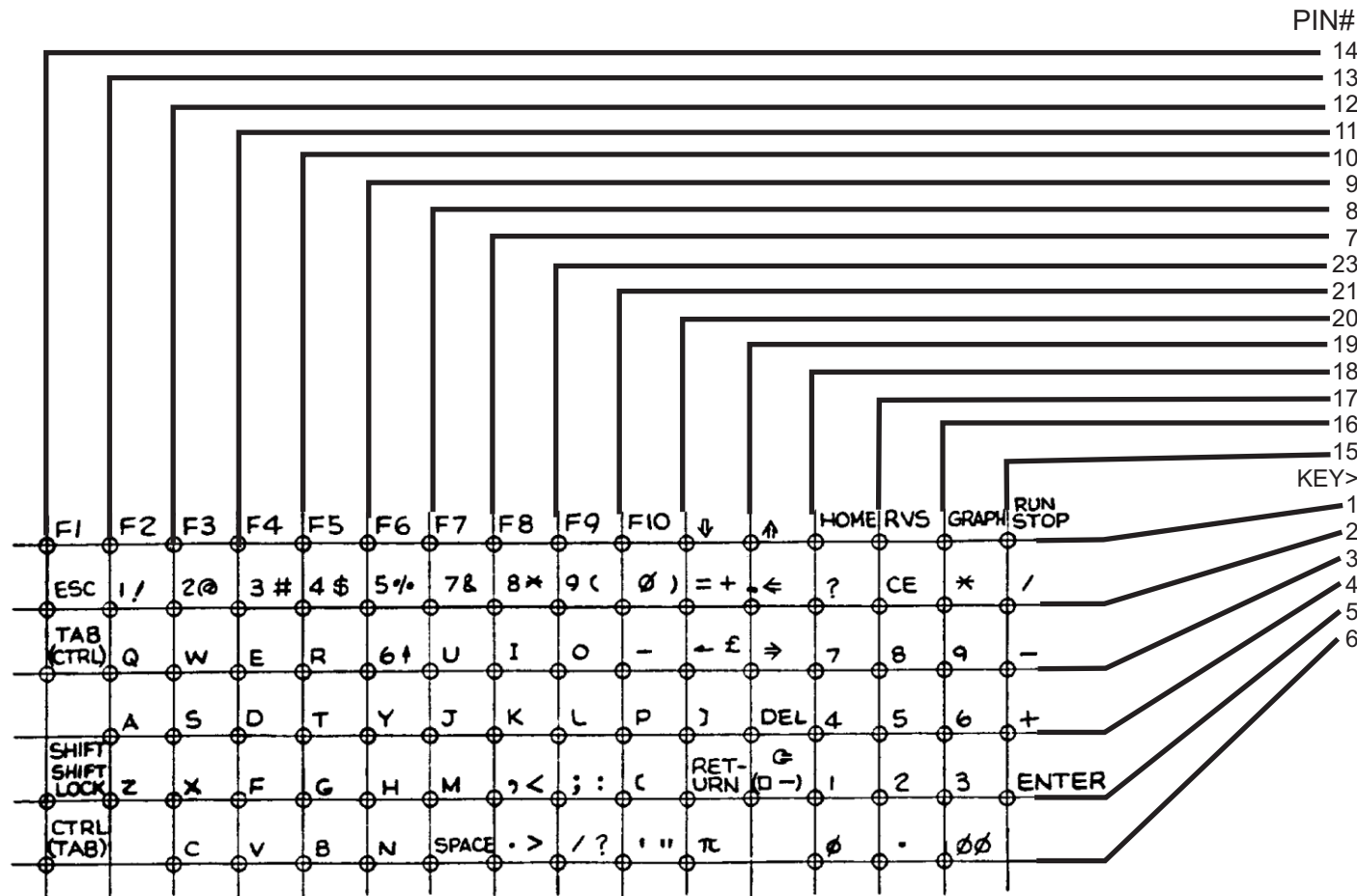
CBM-II Keyboard - PCB connector
