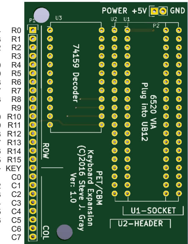
Keyboard Expansion PCB
