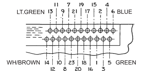
CBM-II Keyboard - PCB connector
